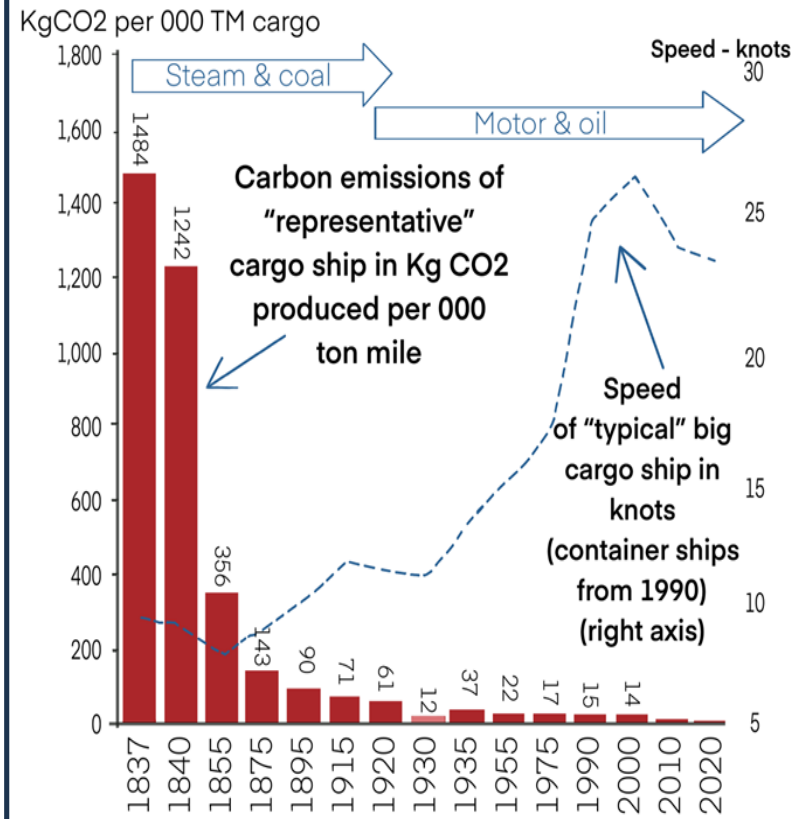
Figure 1: 200 years of bigger ships and smaller emissions Source: Prof. Ian Buxon, Martin Stopford
